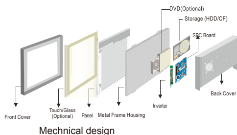
Mechanical design
