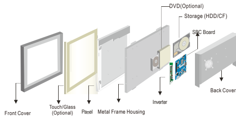
Mechanical design
