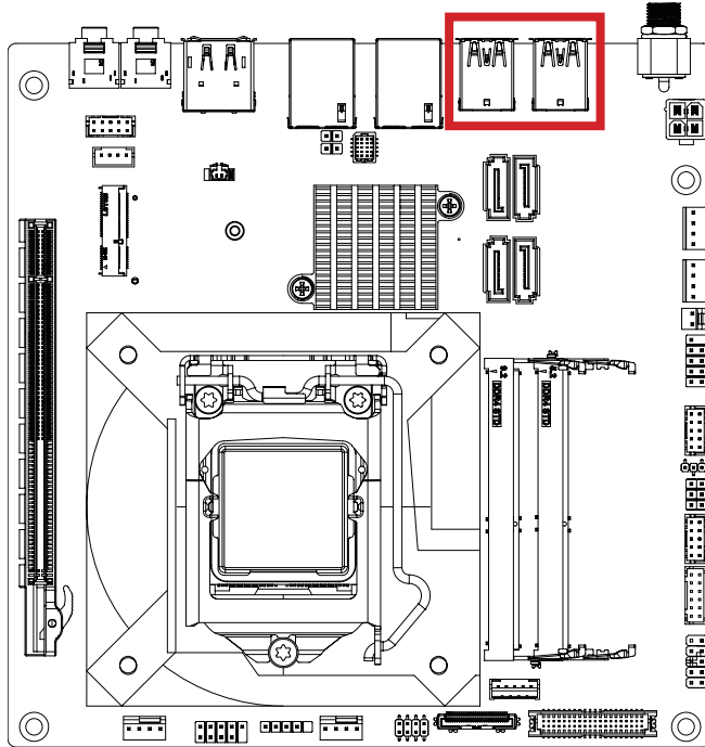
USB Connector
