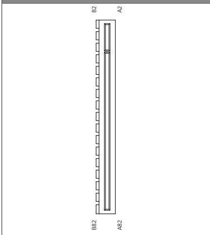
PCIEX16 connector
