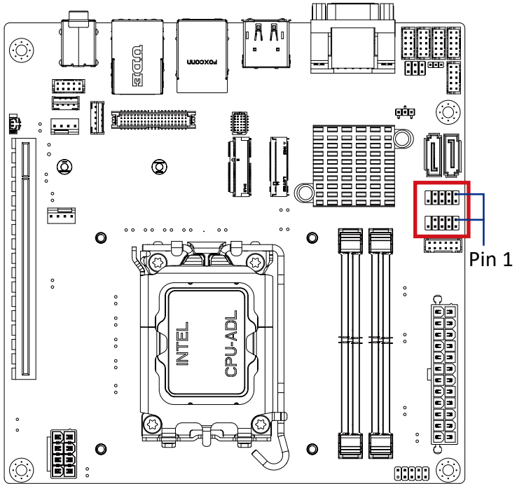
USB 2.0 Header
