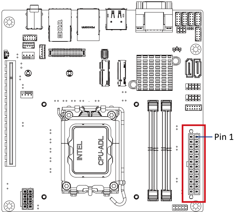
ATX power Connector
